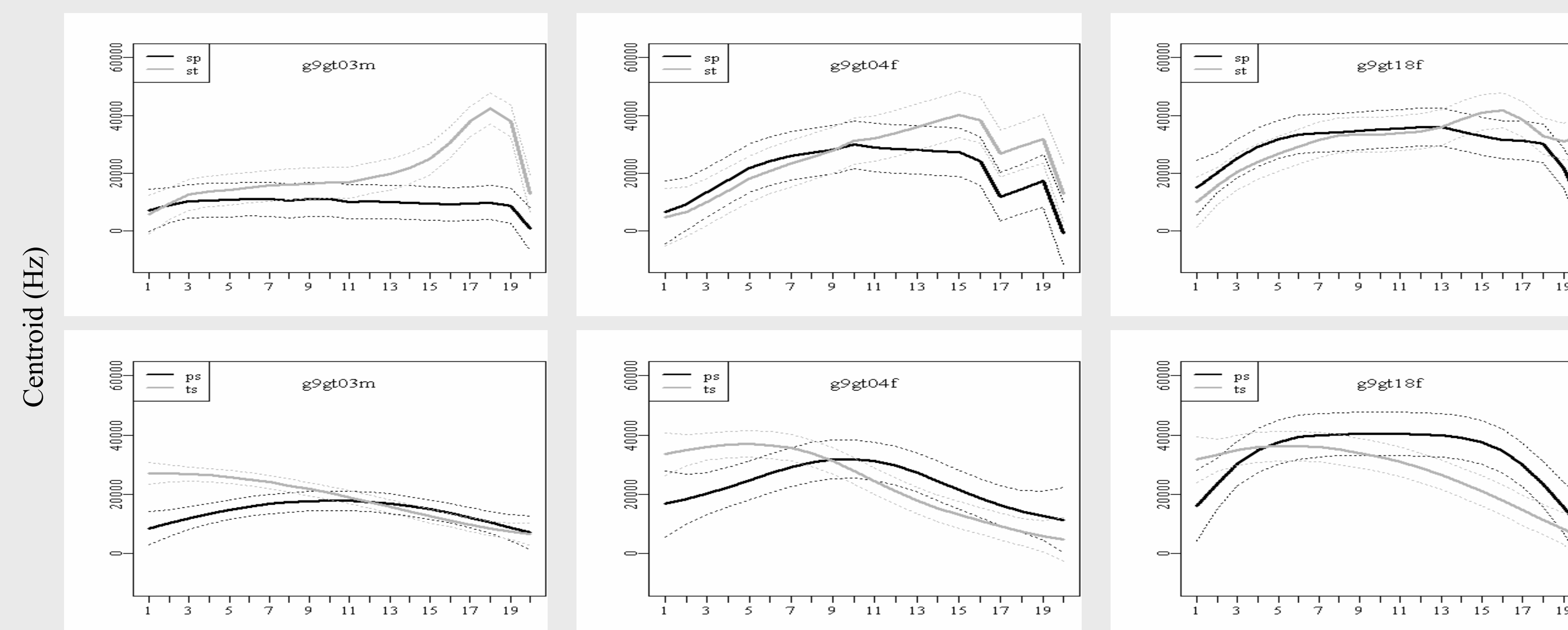
Figure 1. Centroid trajectories of Greek /s/-stop (top) and stop-/s/ sequences (bottom) elicited at word-initial position by 3 Greek adult speakers. The abscissa represents the scaled 20 frames of analysis windows arranged in time sequence, and the ordinate represents the centroid frequencies (first spectral moment). Each solid trajectory line shows the smoothed mean values of the centroid frequencies measured in the /s/-stop and stop-/s/ sequences. The dotted lines below and above the solid line are the 95% confidence intervals.
