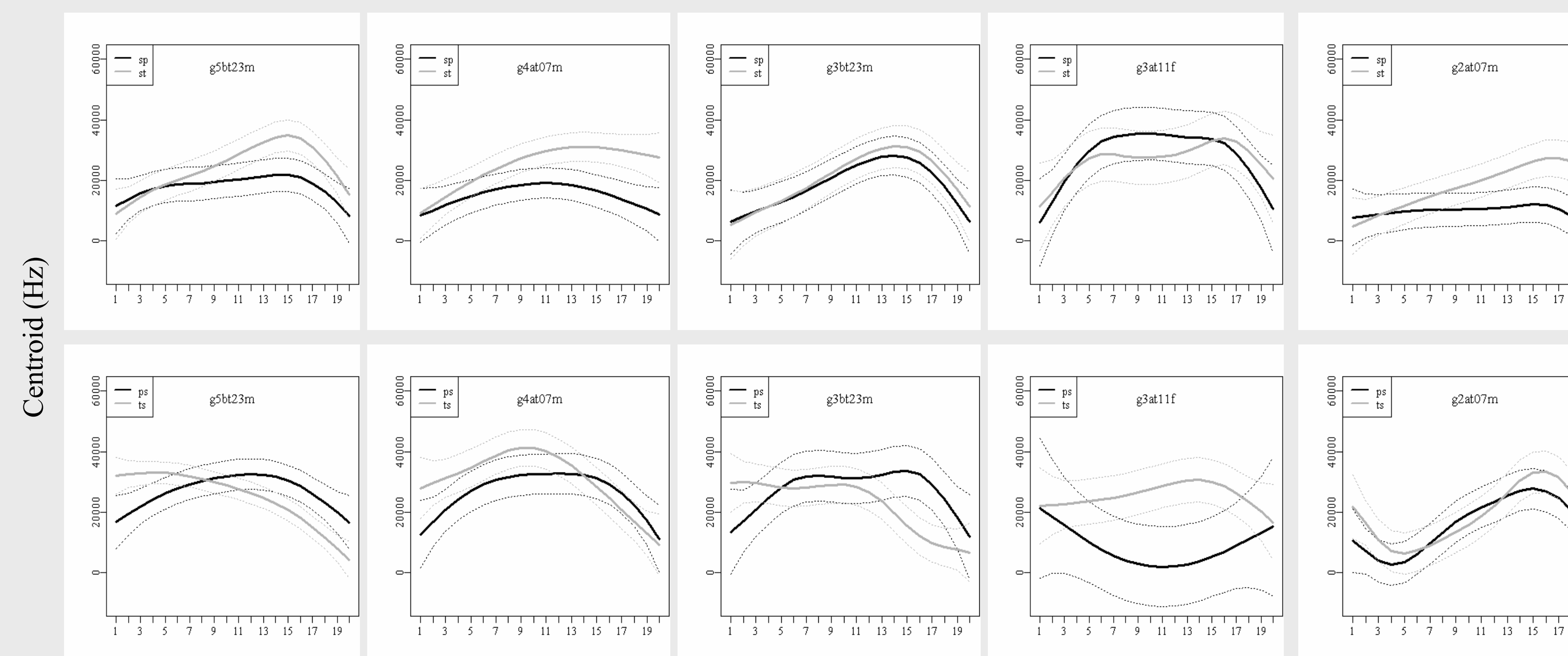
Figure 2. Centroid trajectories of Greek /s/-stop (top) and stop-/s/ sequences (bottom) elicited at word-initial position by Greek child speakers. The abscissa represents the scaled 20 frames of analysis windows arranged in time sequence, and the ordinate represents the centroid frequencies (first spectral moment). Each solid trajectory line shows the smoothed mean values of the centroid frequencies measured in the /s/-stop and stop-/s/ sequences. The dotted lines below and above the solid line are the 95% confidence intervals.
