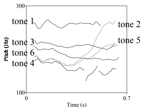
Figure 1. F0 contours for six words [wej] with different tones. Numbers to the right identify the endpoints of the two rising tones (in grey) and numbers to the left identify starting points of the other four tones (in black). The discontinuities in wai4 are where the speaker breaks into creak.
