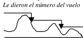
b. schematic representation of downstep
