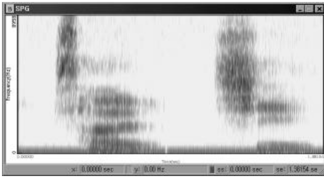
Figure 1. Spectrogram of Korean /sal/ and /si/ [ɕi].
