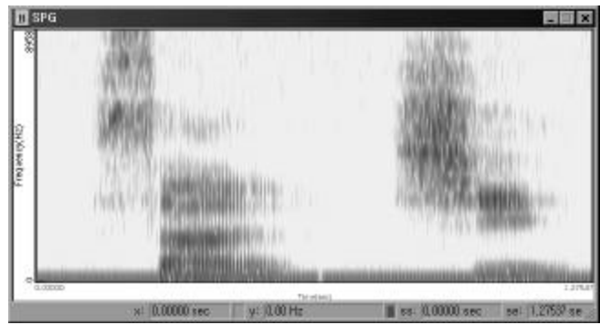
Figure 2. Spectrogram of Korean /s'al/ and /s'i/ [ɕ'i].
