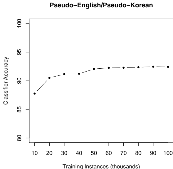
Figure 2: Classifier accuracy trained on pseudo-English loanwords and pseudo-Korean items; classifying actual English and Korean words.
