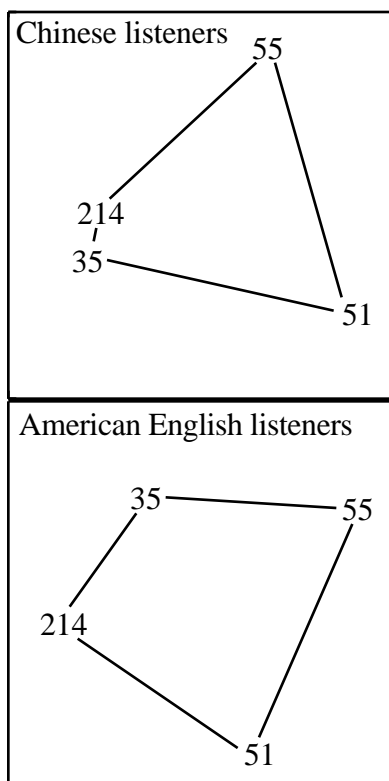
Figure 1. The four tones of Mandarin Chinese in perceptual space for Mandarin Chinese listeners and American English listeners. Multidimensional scaling data from Huang (2000).
