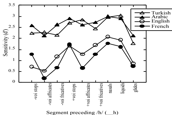
Figure 6. Perceptual sensitivity to /h/ in different segmental contexts by listeners of American English, Turkish, Arabic, & French. Data from Mielke (2000).
