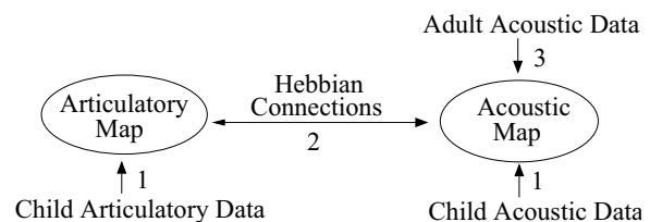
Figure 1: Model Components. We present associated child data points to the articulatory and acoustic maps (1). We then update the Hebbian connections between the two maps (2). We alternate babbling training with listening training, (3), in which adult acoustic data is presented to the acoustic map only.
