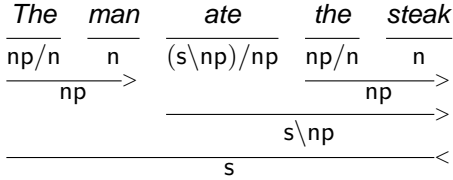
Figure 1: A simple CCG derivation, showing how CCG categories combine to make a sentence.
