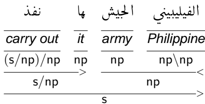
Figure 17: The prediction of the basic algorithm on the somewhat exceptional case of VOS word order, where the object is generally a pronominal suffix. The sentence means the Philippine army carried it out .
