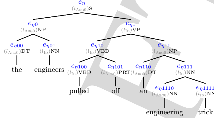
FIGURE 2 Syntax and semantics annotated on a tree. Referents e are subscripted with the node’s address. Relations l and syntactic categories c are specific to the example; the relation ARG0 indicates that the NP is the 0 th argument of S, and ID shows that the VP is the main predicate of S.
